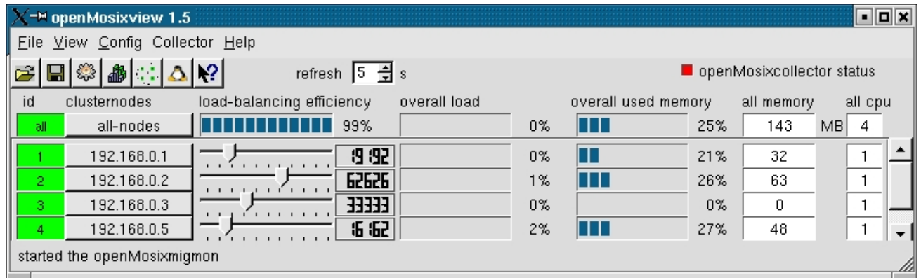
Figura C.2: openMosixview-finestra principale
